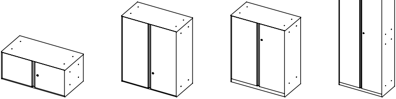
Upper 上置 W900 D450 H386/724/1076 Base 下置 W900 D450 H784/1136/2212
