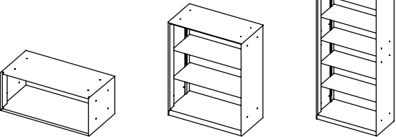
Upper 上置 W900 D450 H386/724/1076 Base 下置 W900 D450 H784/1136/2212
